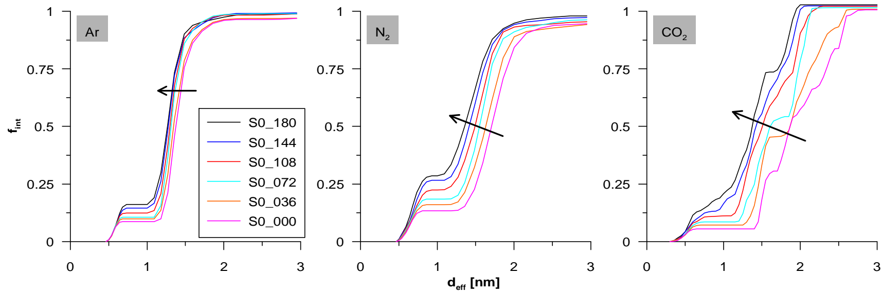
Figure S1. The comparison of the plots of integral pore size distributions from figure 5.
