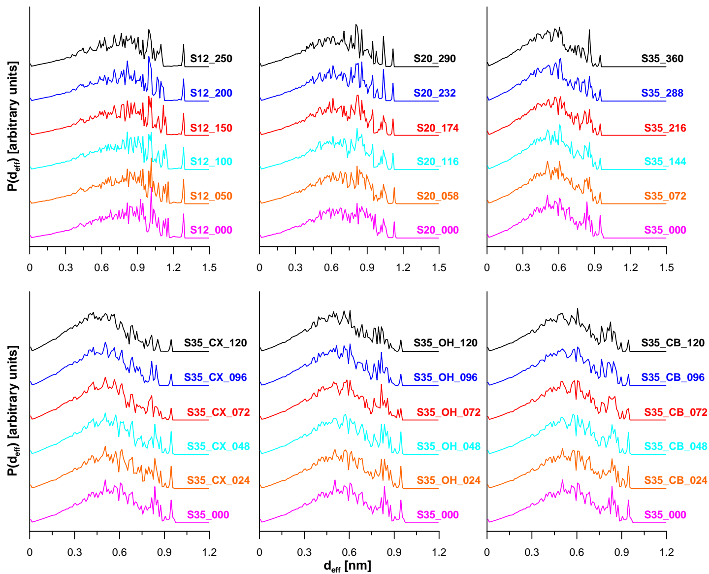
Figure S1. Histograms of the pore diameters obtained from BG method.
