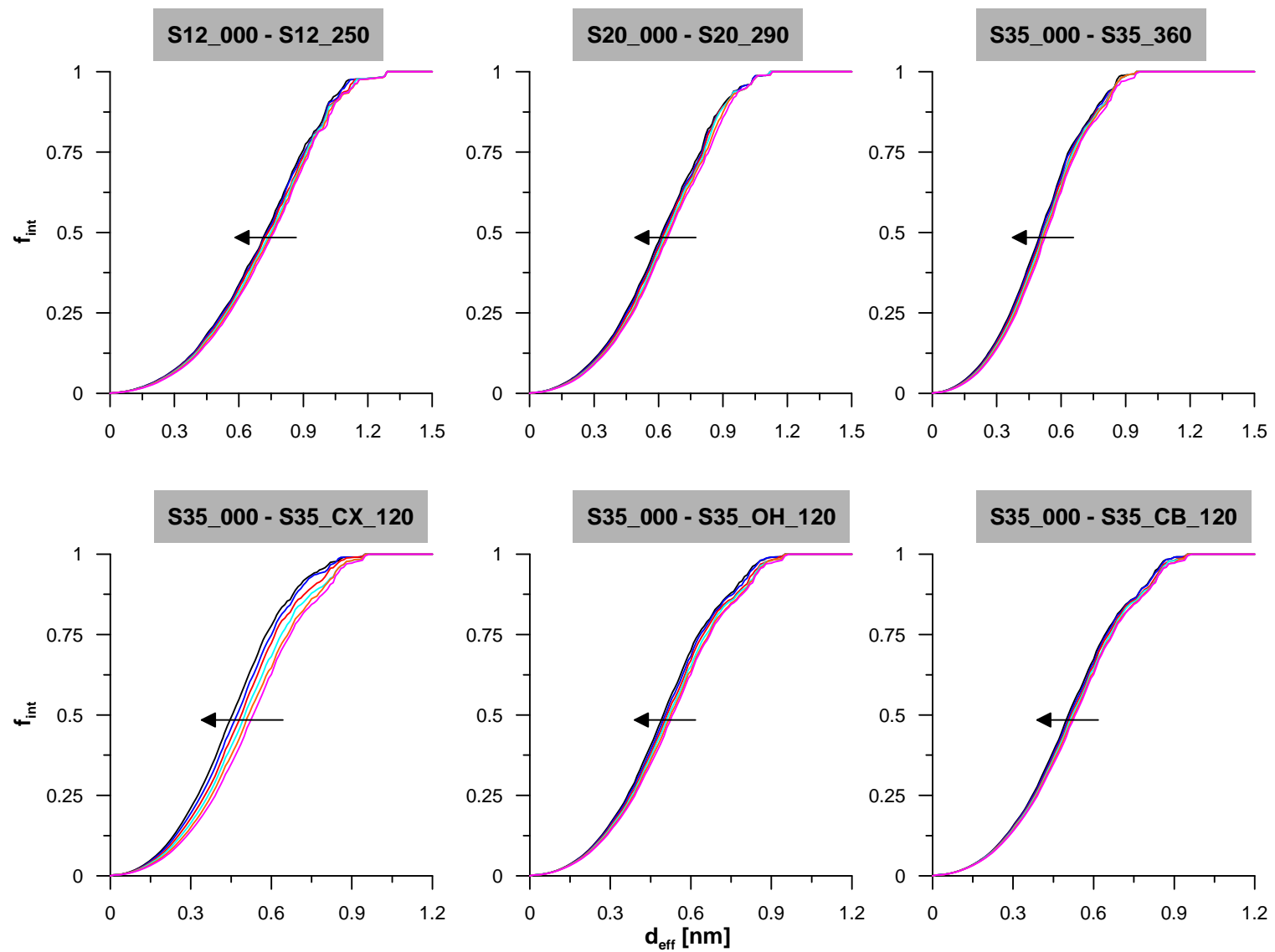
Figure S2. Cummulative PSDs from the BG method (arrows show the rise in the number of groups).
